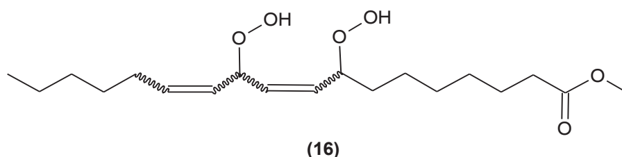
Figure 27: Structural formula of methyl 8,11-bishydroperoxyoctadeca-9,12-dienoate (16).
